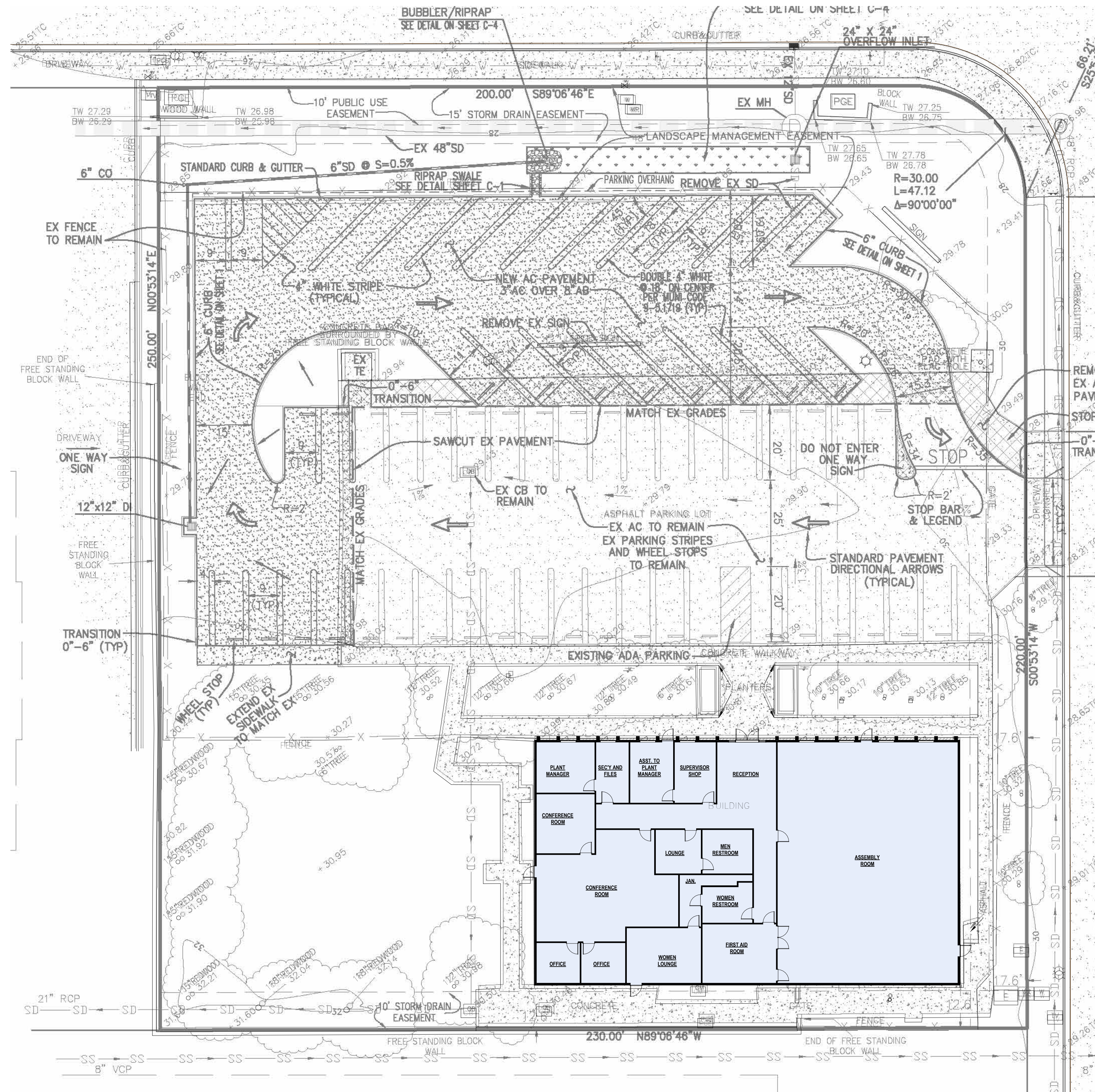
EXISTING BUILDING 1/16" = 1'-0" 1
