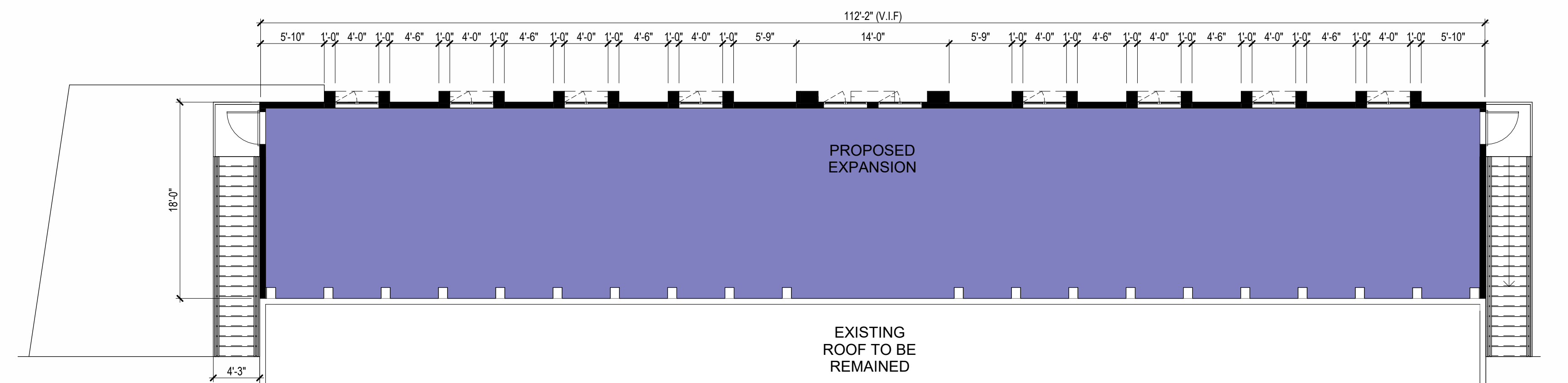
LEVEL 2 EXPANSION FLOOR PLAN 1/8" = 1'-0" 2
